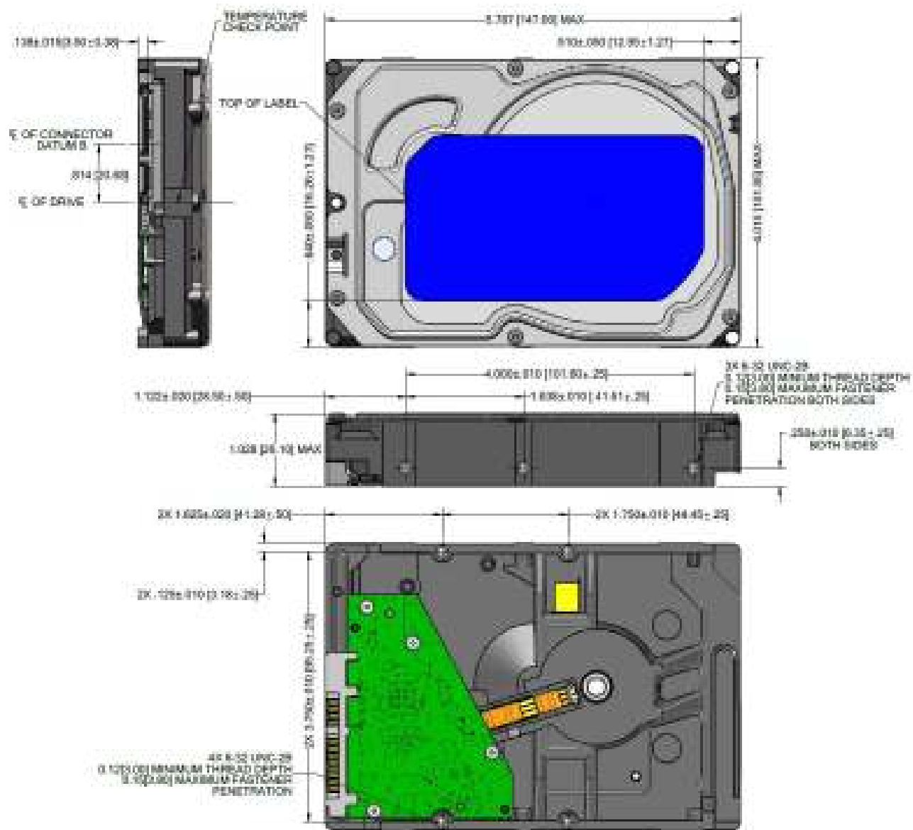
Figure 3 Mounting dimensions (3 and 4-disk models)
