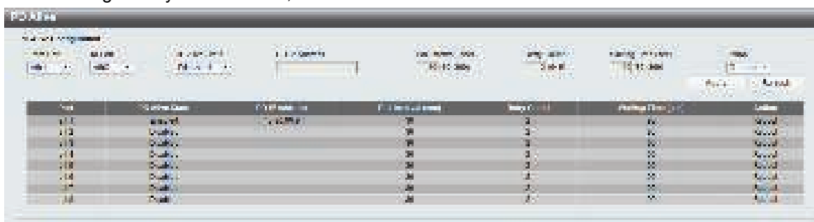
Figure 4.19 – System > PoE > PD Alive
