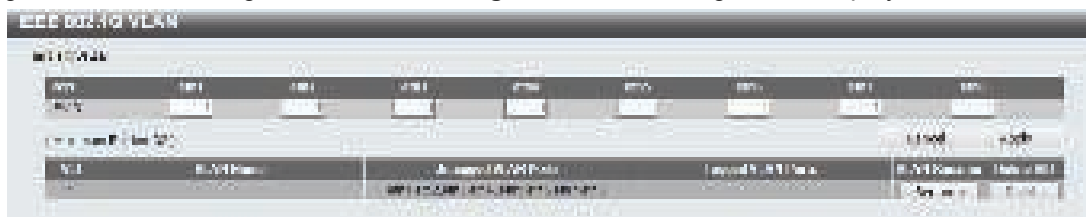
Figure 4.31 – L2 Features > VLAN > 802.1Q VLAN – PVID Settings
