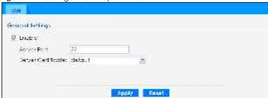
Figure 122 Configuration > System > SSH
