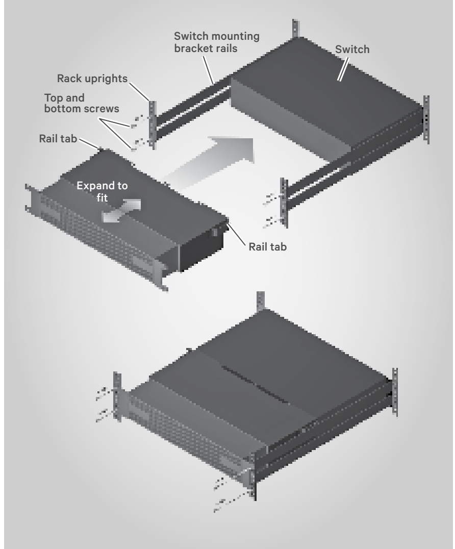
Geist SwitchAir Rack Installation
