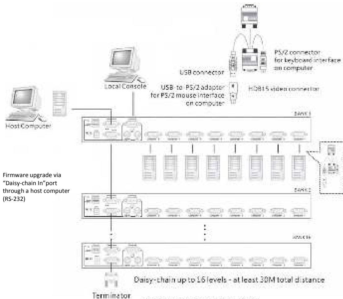
Configuration Diagram
