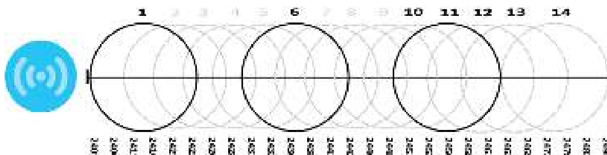
Figure 160 An Example Three-Channel Deployment
