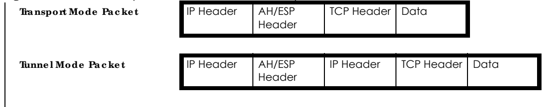
Figure 280 VPN: Transport and Tunnel Mode Encapsulation
