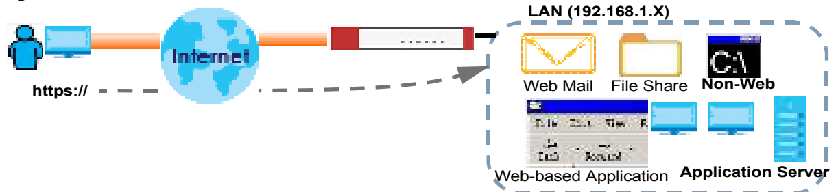
Figure 265 SSL VPN
