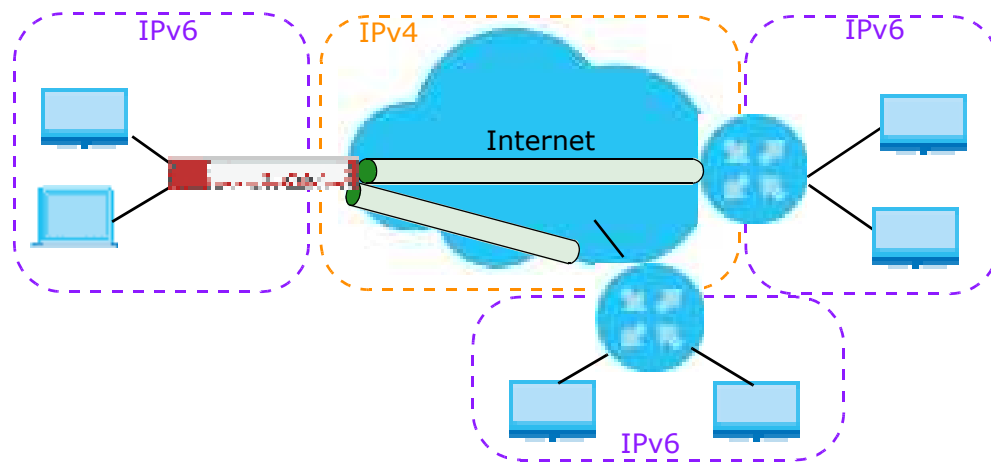
Figure 183 6to4 Tunnel
