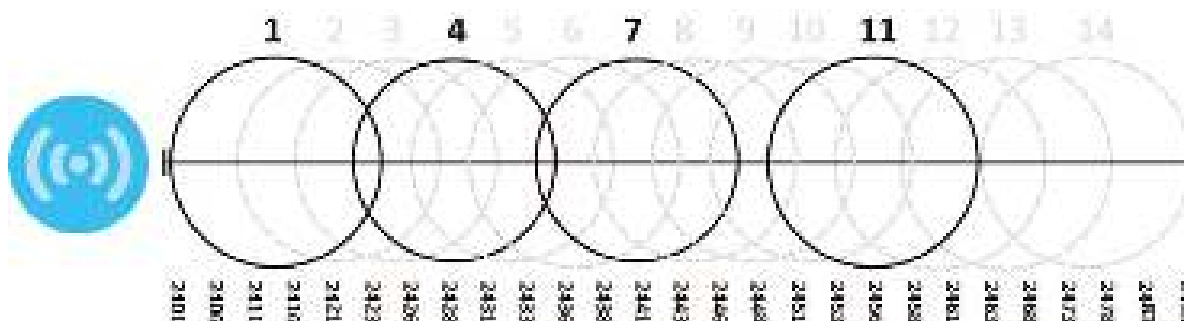
Figure 161 An Example Four-Channel Deployment
