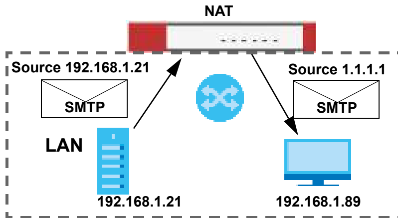
Figure 229 LAN to LAN Return Traffic
