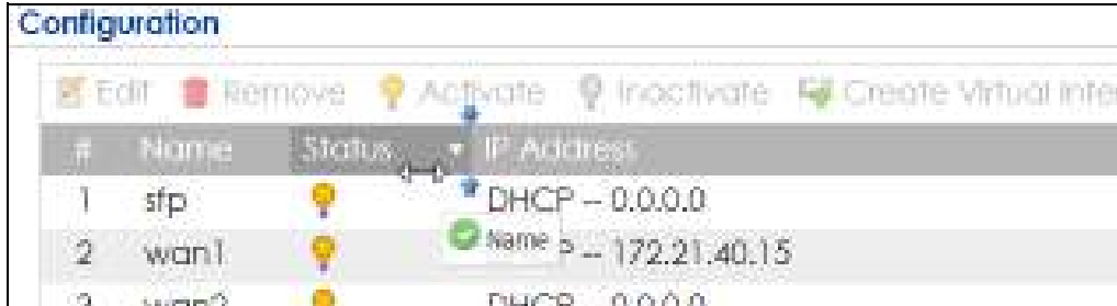
Figure 18 Moving Columns
