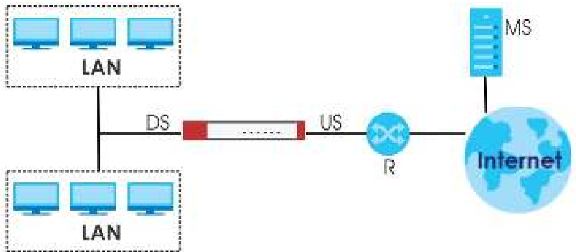
Figure 165 IGMP Proxy
