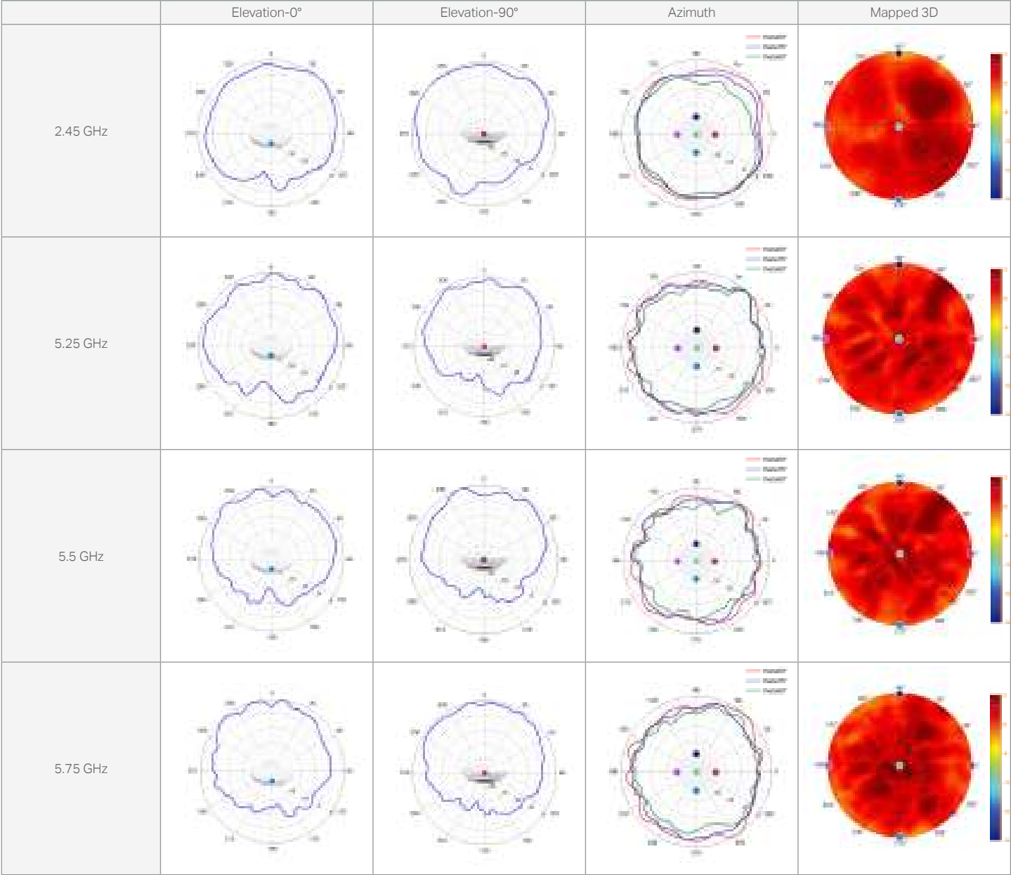
EAP660 HD
