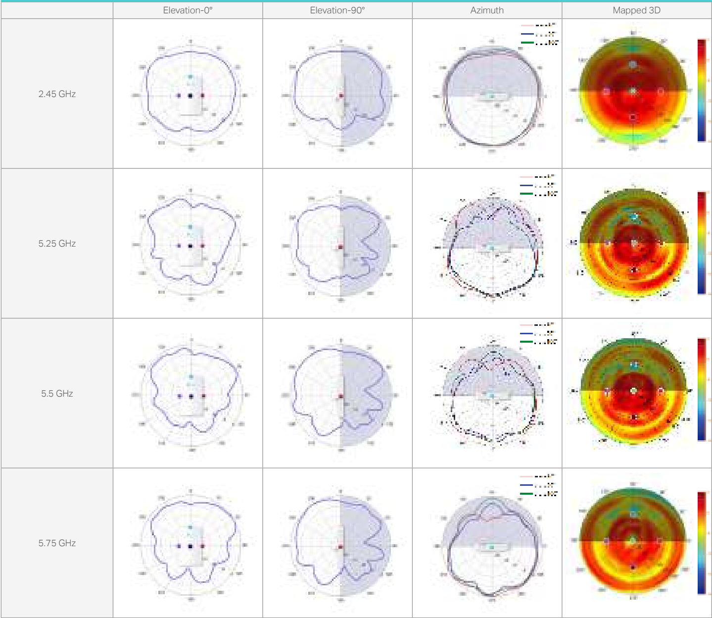
EAP225-Wall
