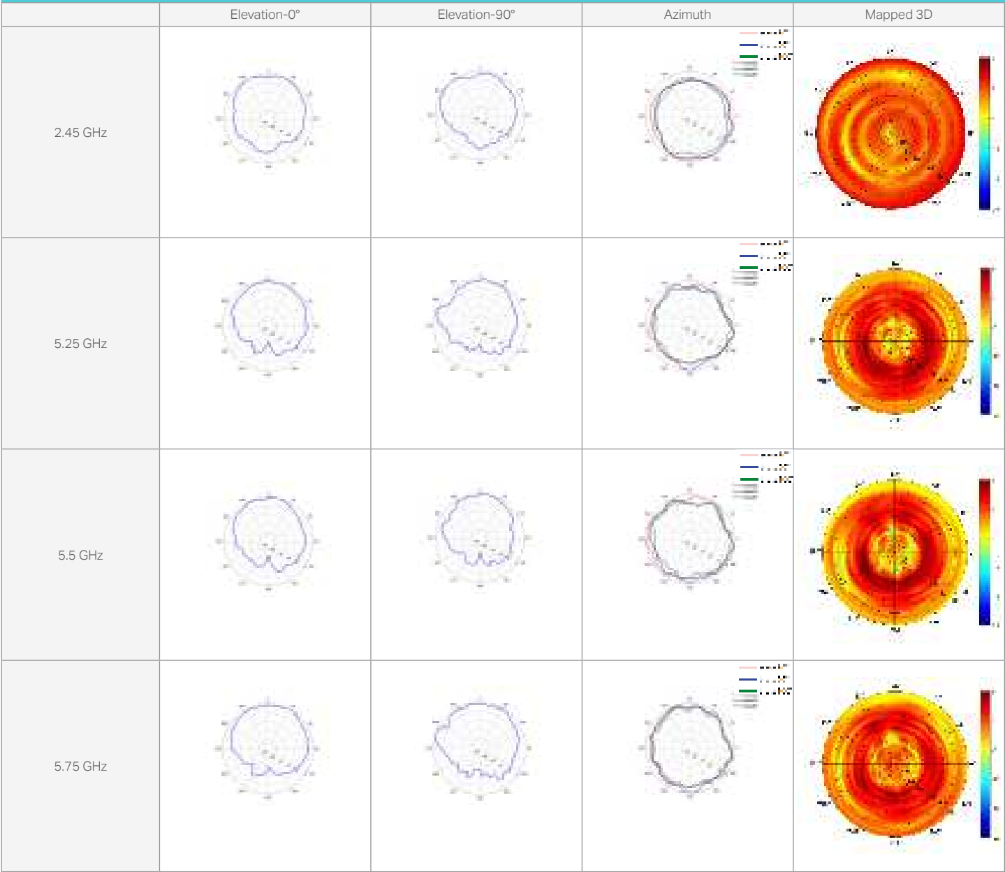
EAP650-Outdoor
