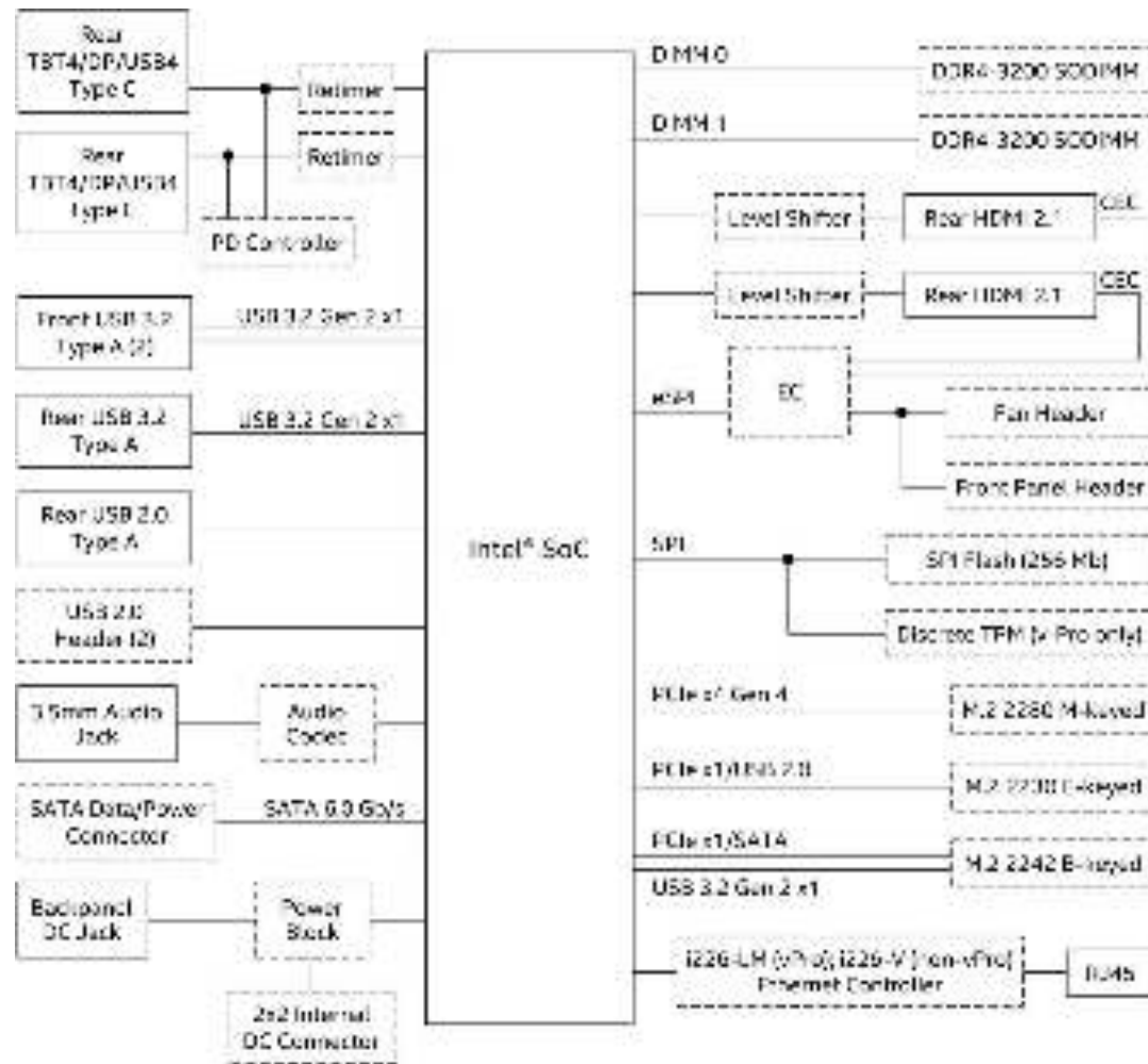
Figure 6. Block Diagram
