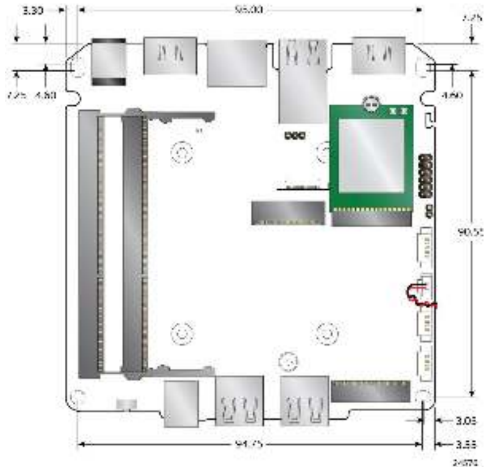
Figure 15. Board Dimensions
