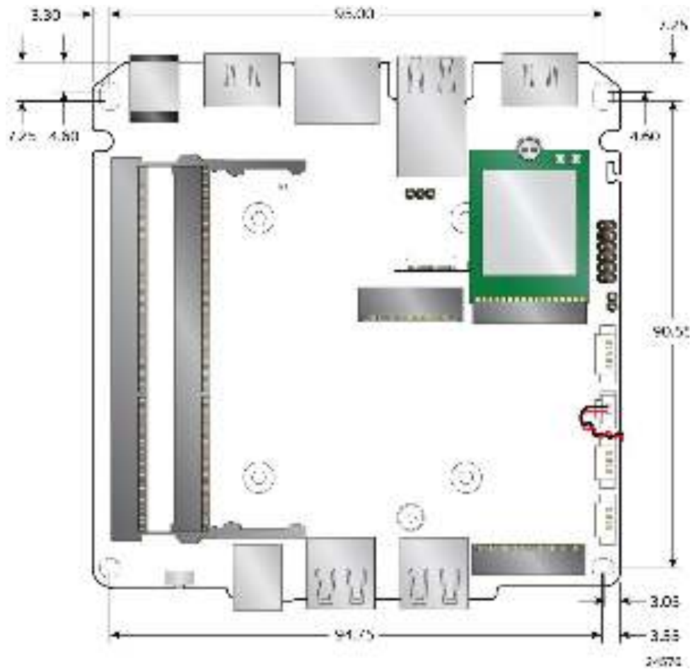
Figure 15. Board Dimensions
