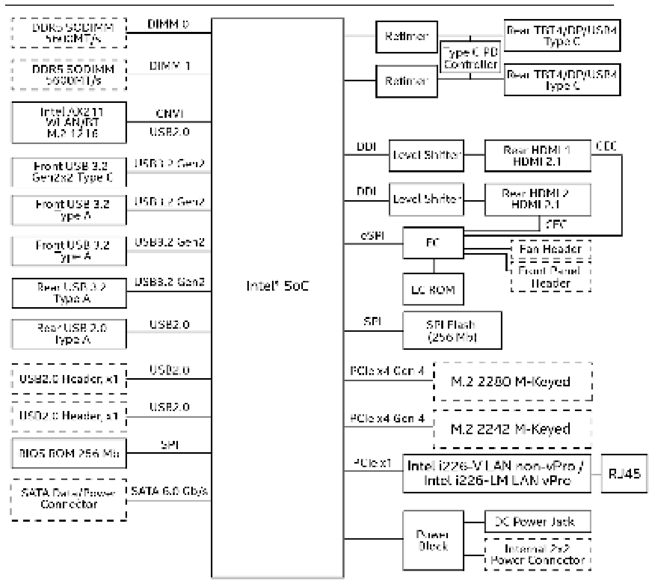
Figure 6. Block Diagram
