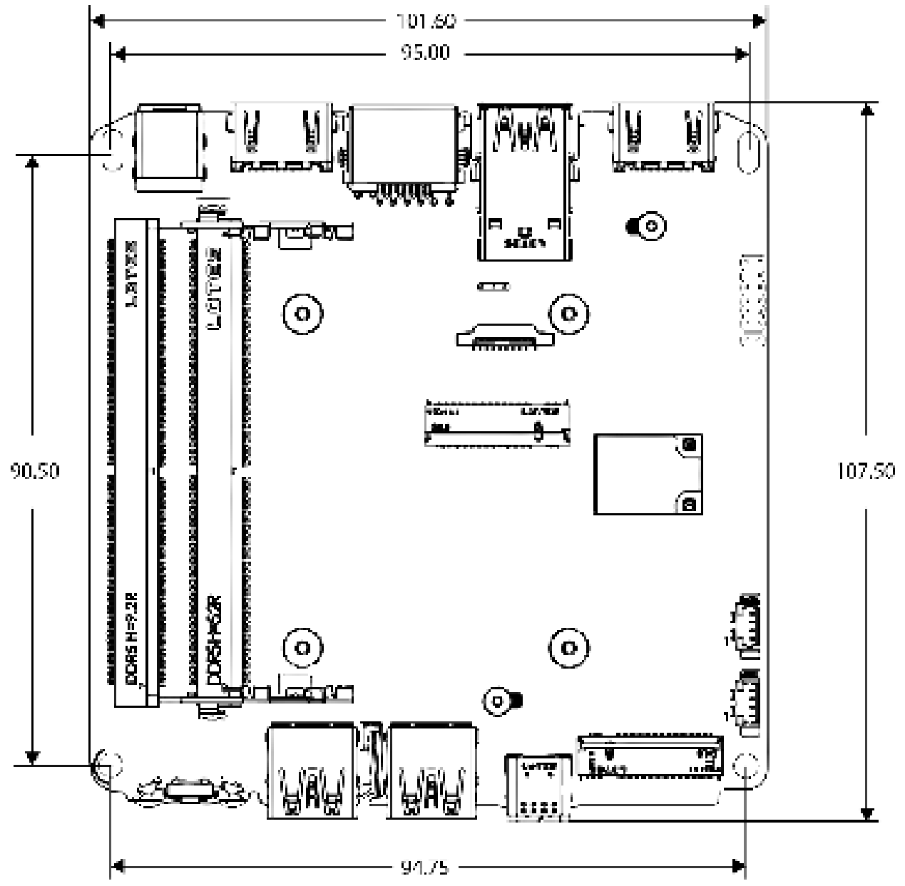
Figure 17. Board Dimensions
