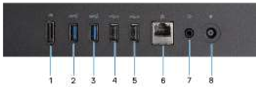
Figure 7. Back panel view of OptiPlex All-in-One 7420 with an Energy Efficient processor
