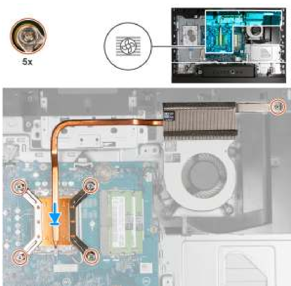
Figure 110. Installing the heat sink
