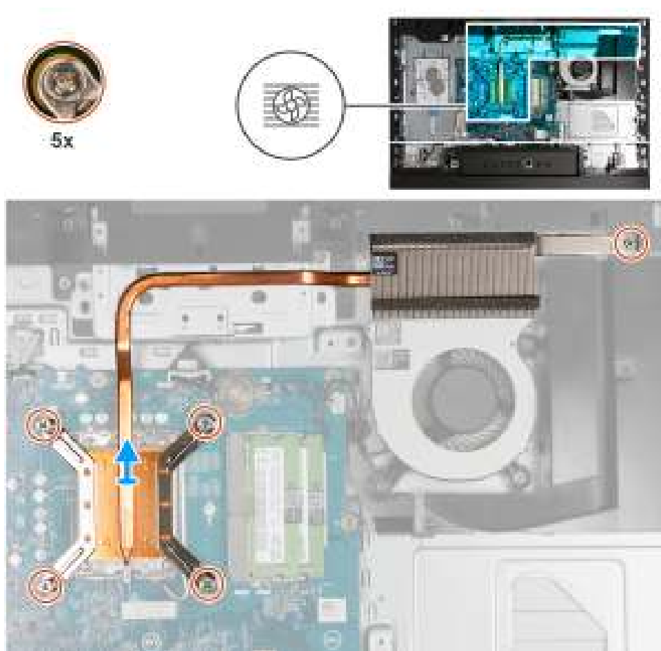
Figure 109. Removing the heat sink
