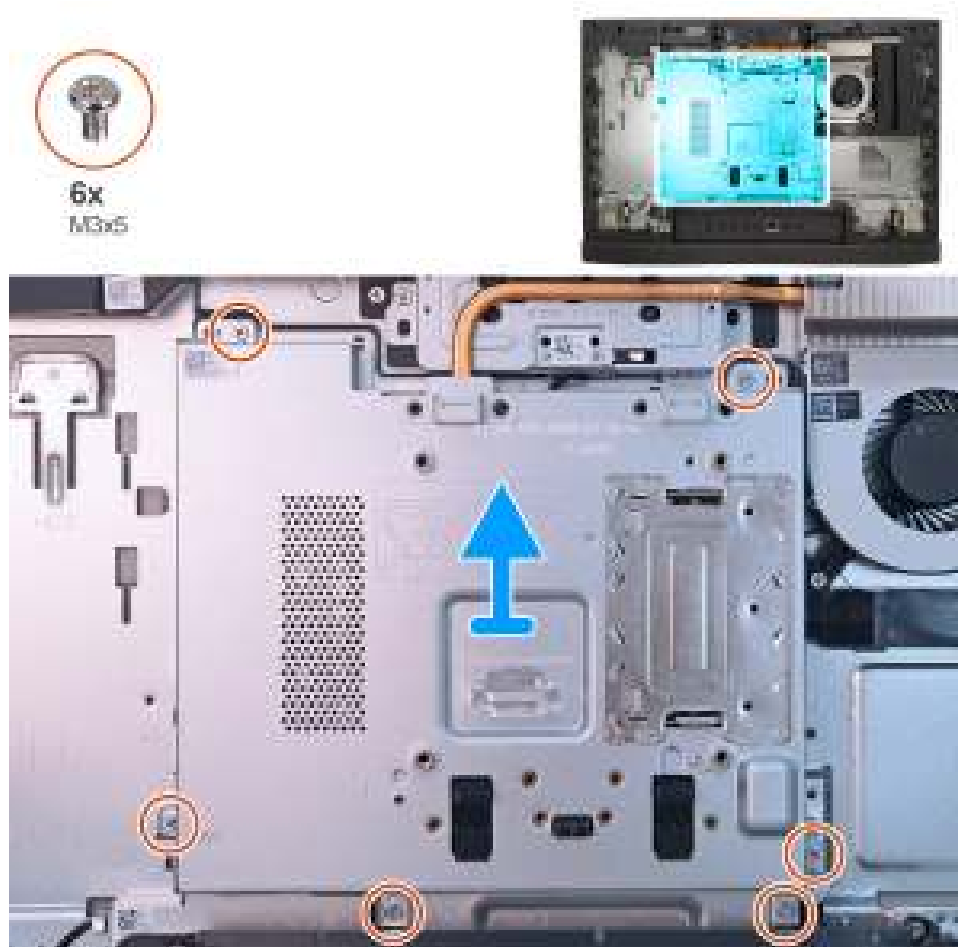
Figure 86. Removing the system-board shield
