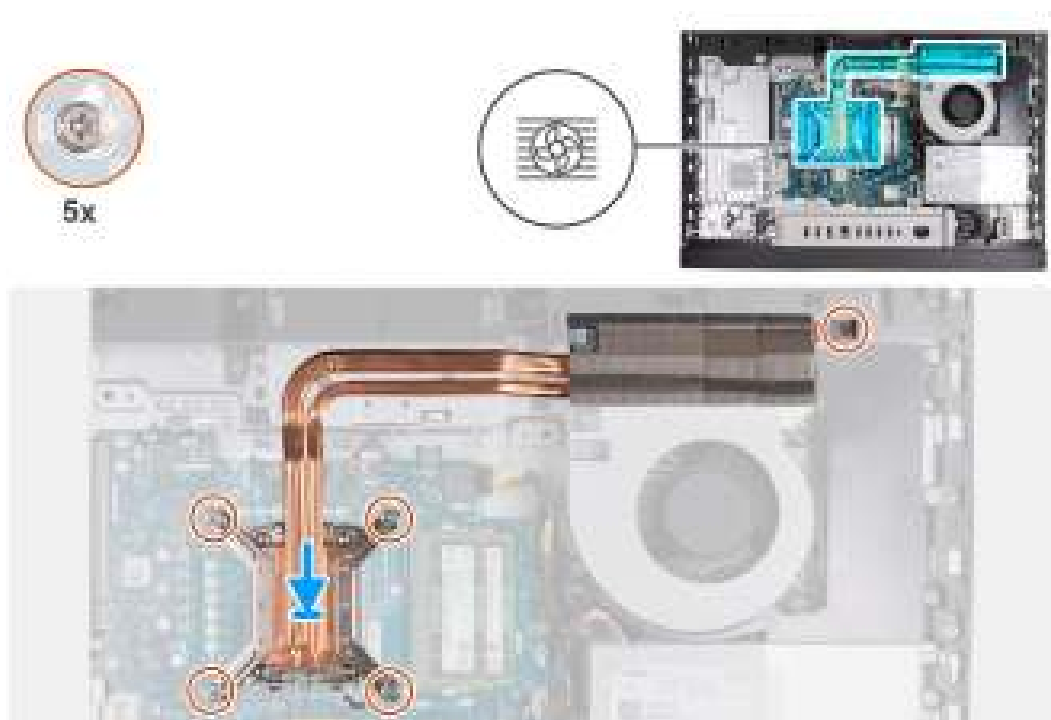
Figure 63. Installing the heat sink
