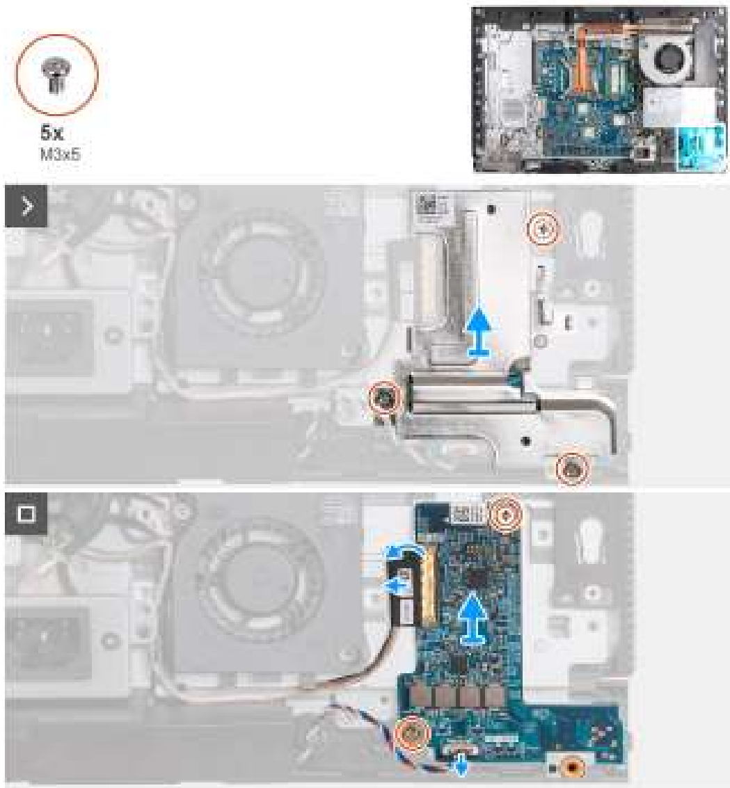
Figure 74. Removing the audio board
