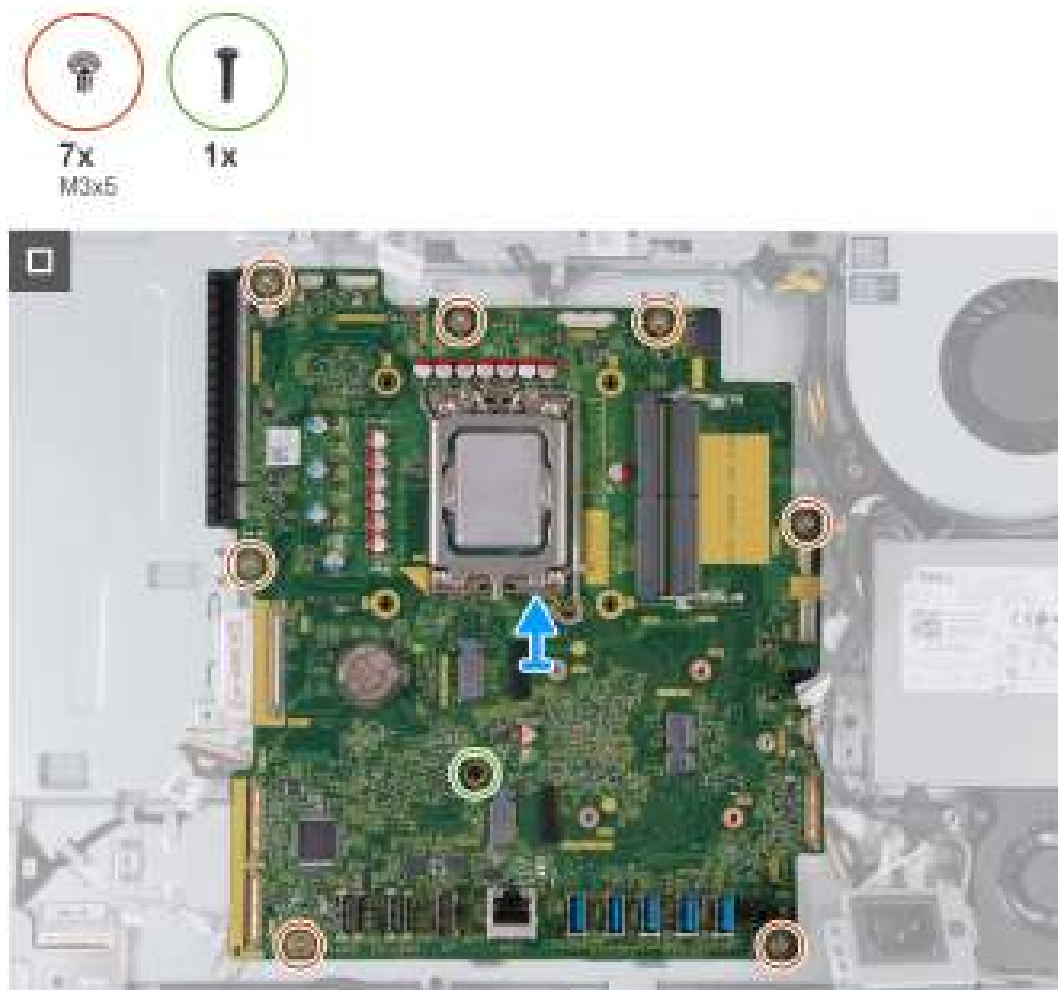
Figure 68. Removing the system board
