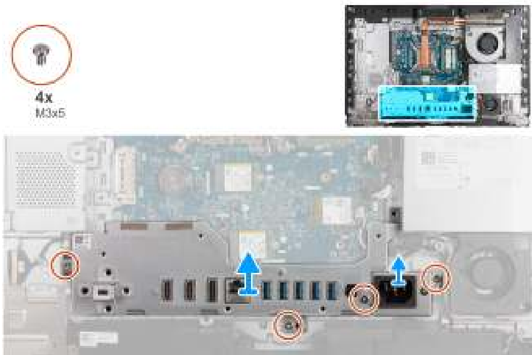
Figure 58. Removing the I/O bracket
