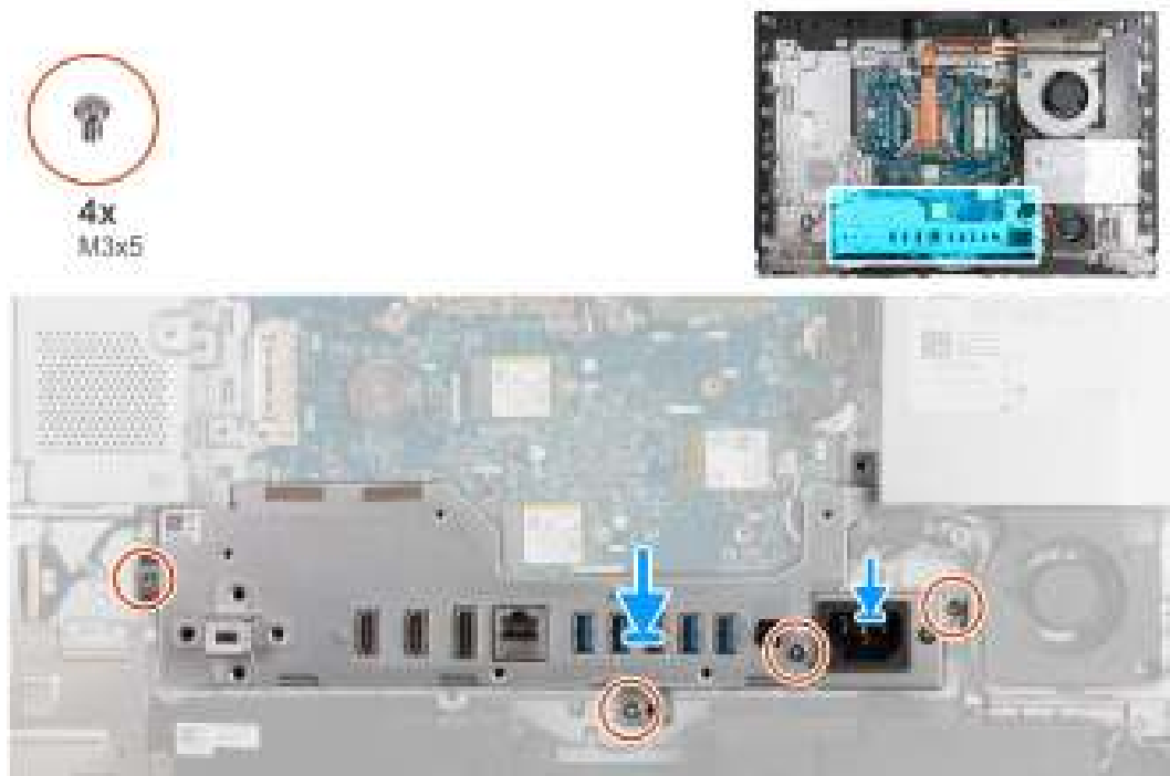
Figure 59. Installing the I/O bracket
