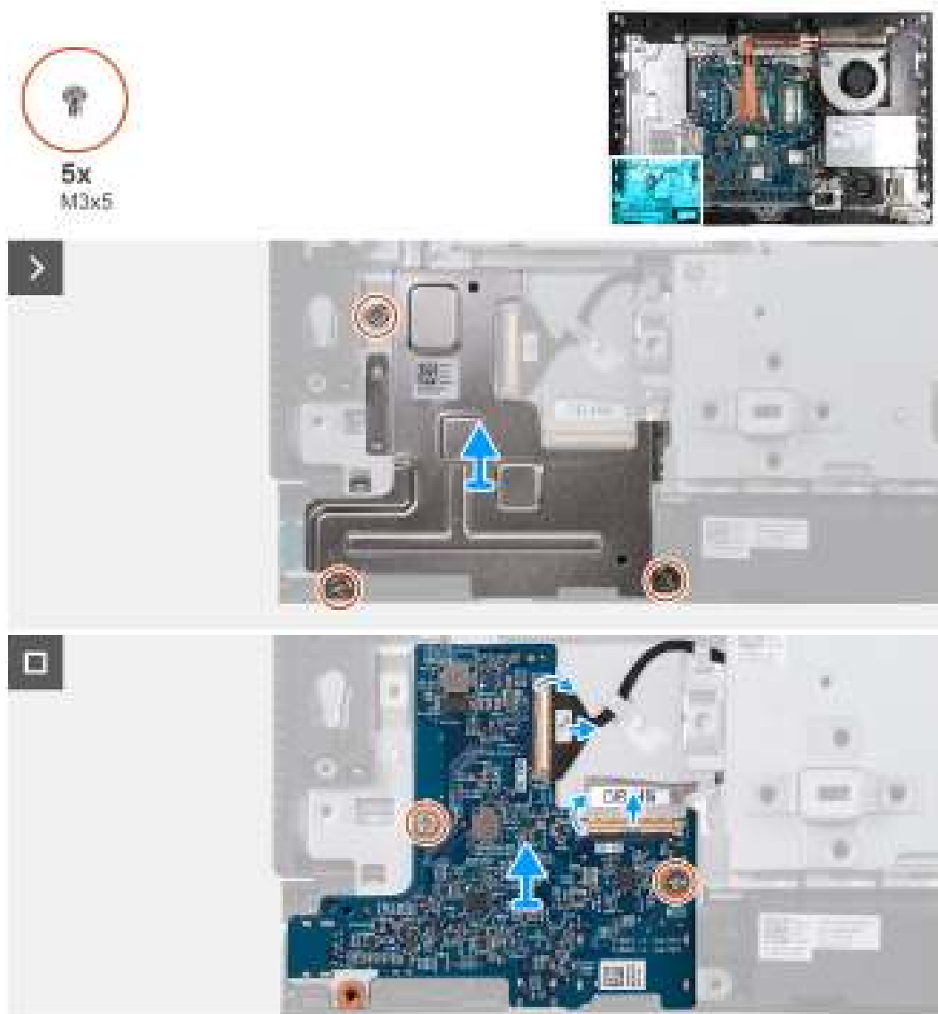
Figure 72. Removing the power-button and I/O board
