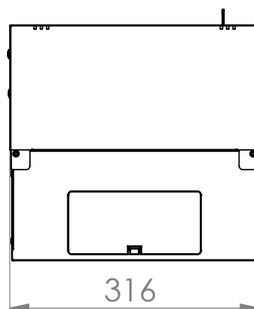
Bottom view
