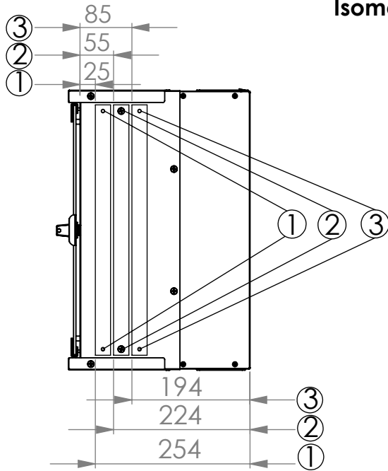
Isometric views
