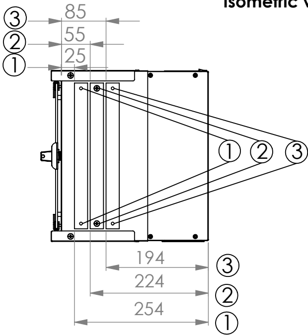
Isometric views
