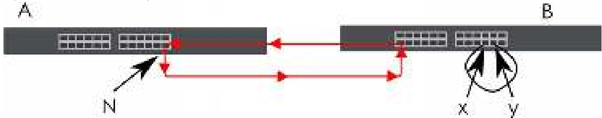
Figure 195 Switch in Loop State
