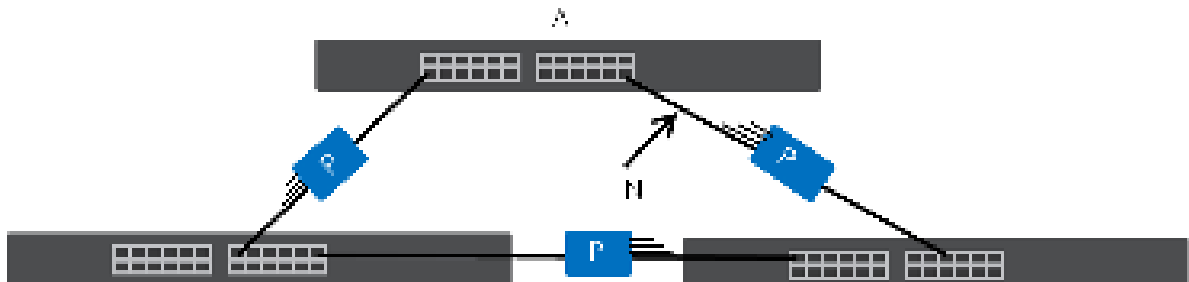
Figure 197 Loop Guard – Network Loop
