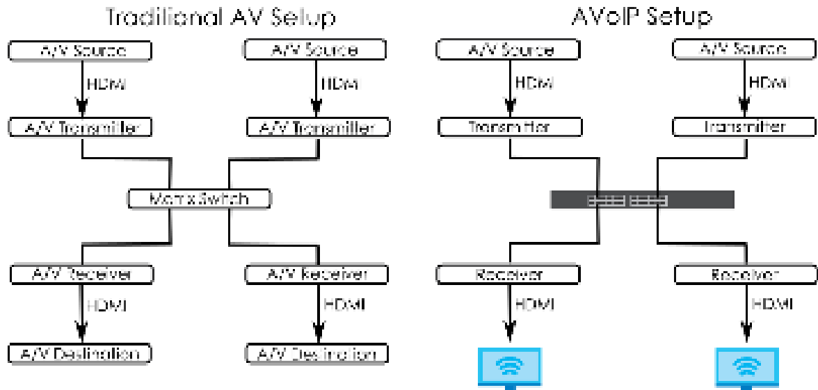
Figure 3 Comparison Between Traditional AV and AVoIP Setups
