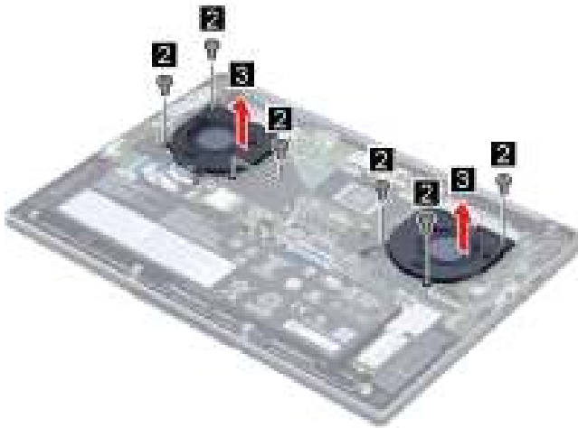
Figure 16. Remove the fans
